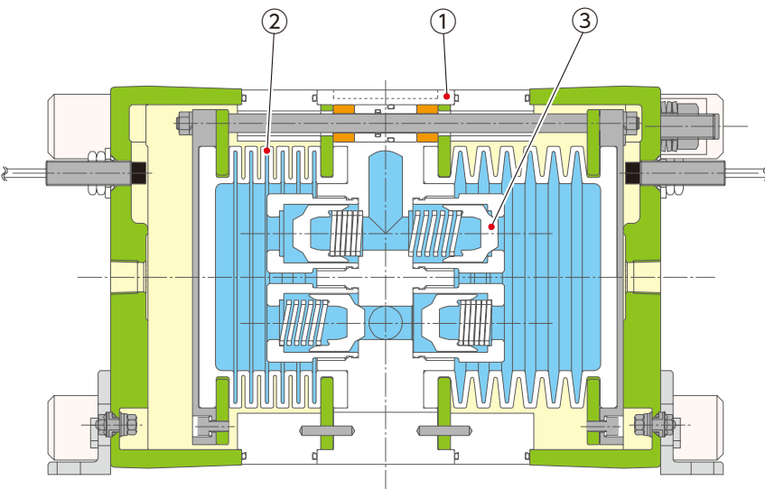
Wetted parts
